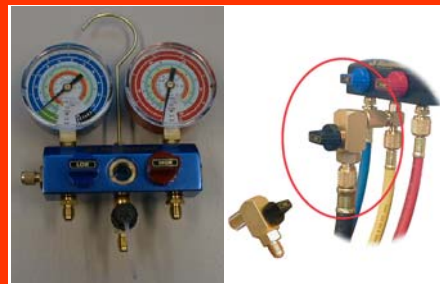
DELUX 3/8 BORE BALL VALVE MANIFOLD GAUGE + ADAPTER P/N TE58103-MRB P/N 90530
